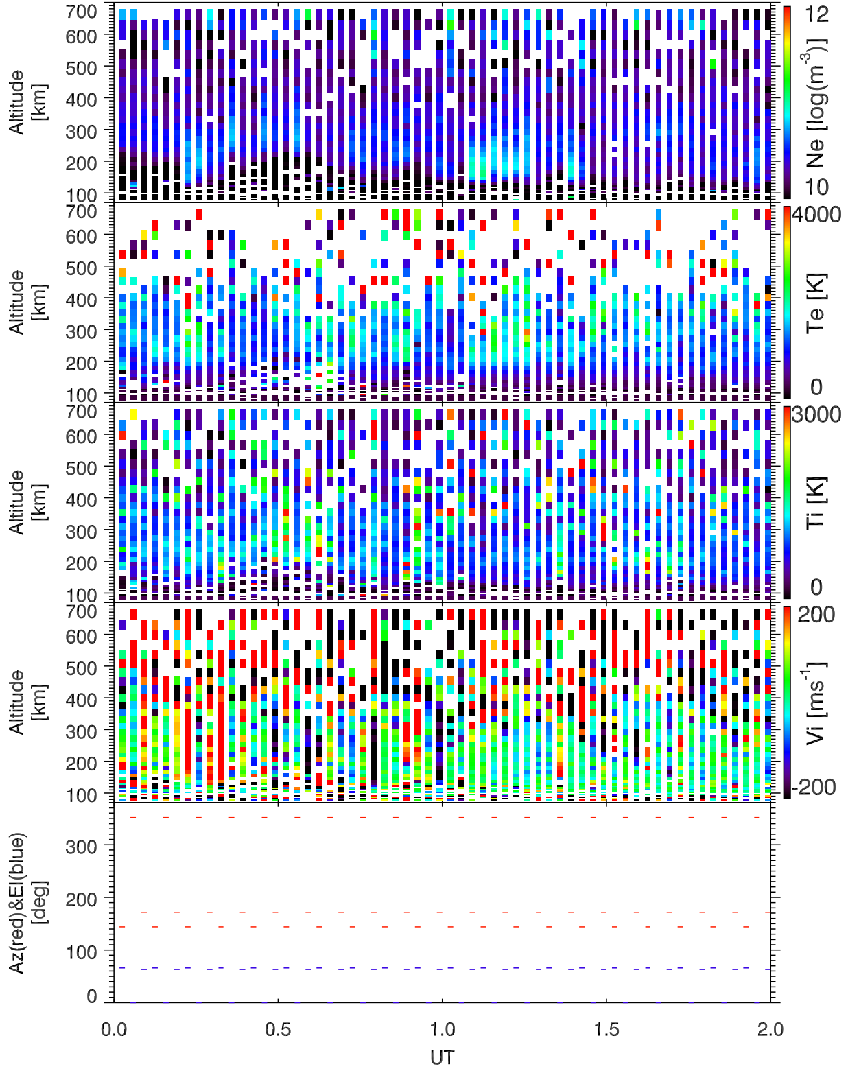
EISCAT 2007-03-03_00_02UT_all_all@32m.
