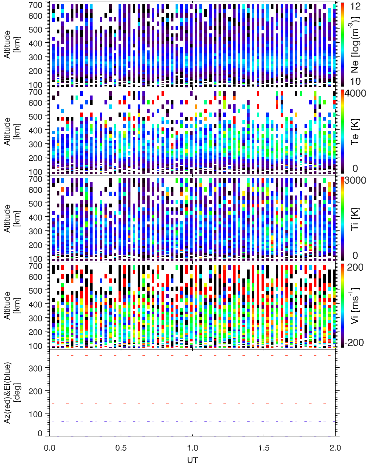
EISCAT 2007-03-04_00_02UT_steffe_ant@32m.
