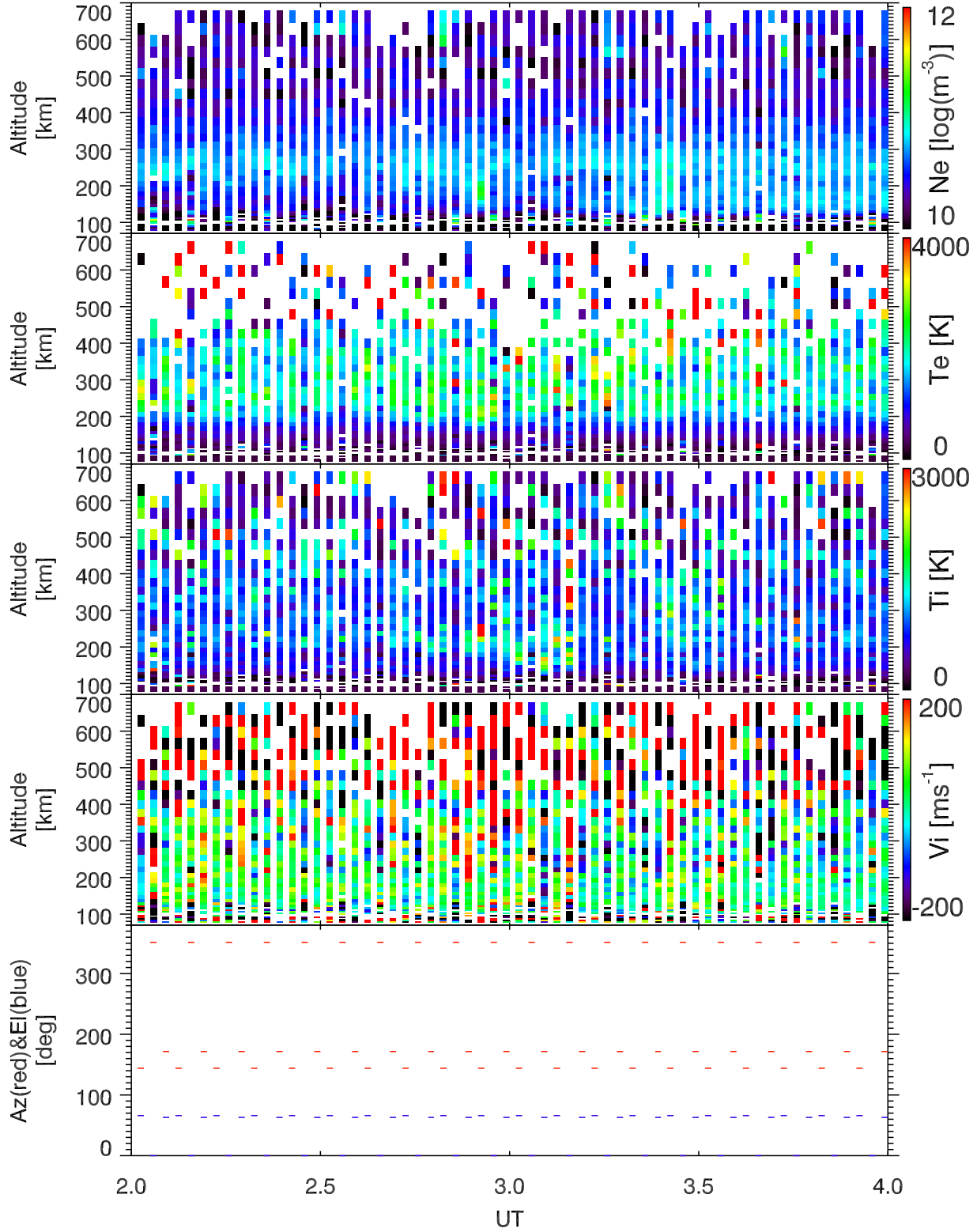
EISCAT 2007-03-04_02_04UT_steffe_ant@32m.
