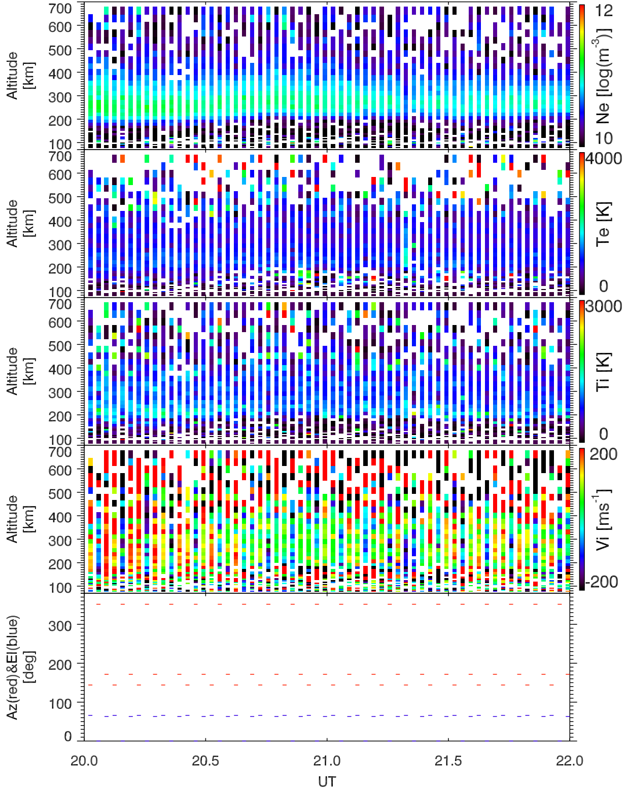
EISCAT 2007-03-04_20_22UT_steffe_ant@32m.
