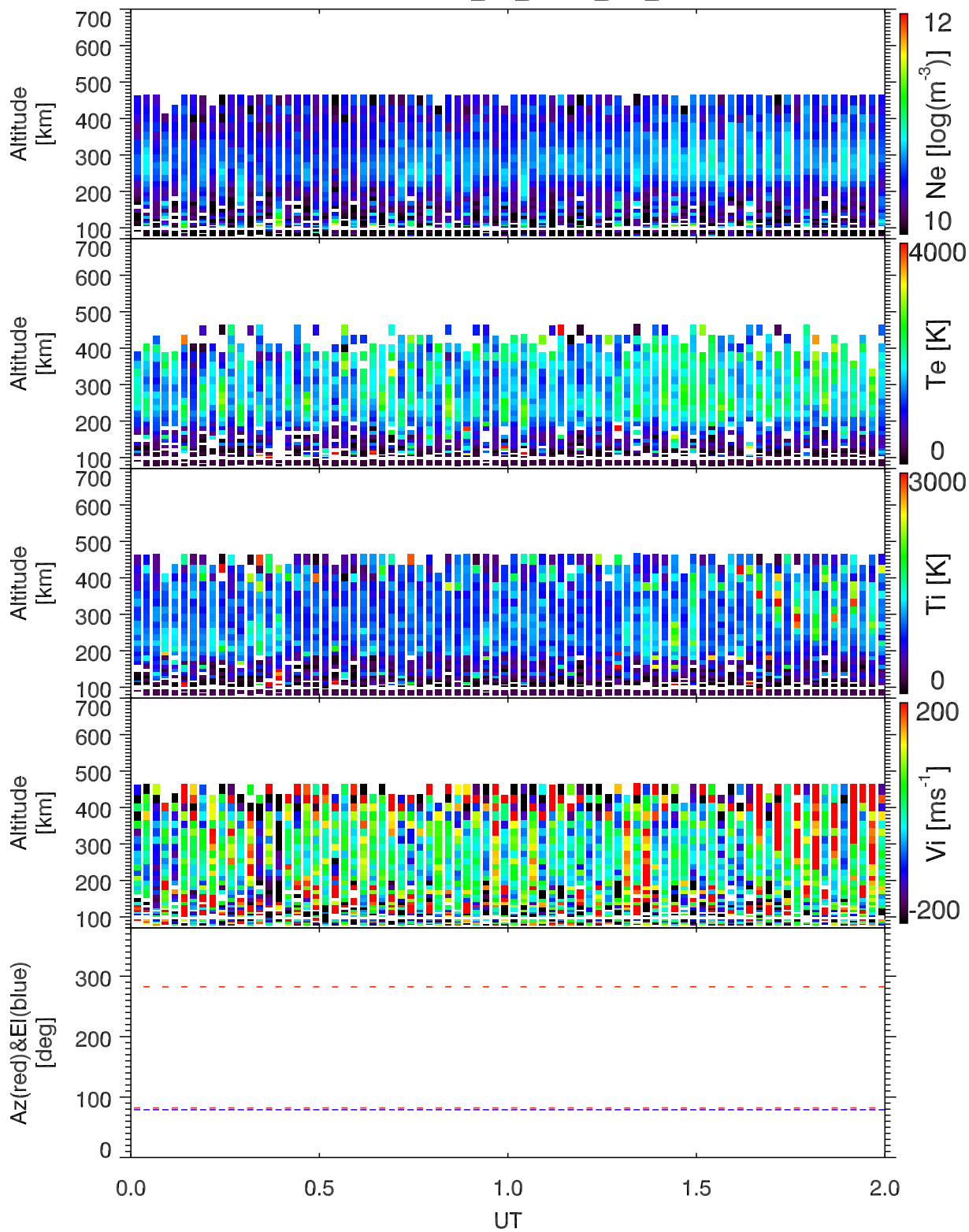
EISCAT 2007-03-21_00_02UT_ipy_ant@32m.
