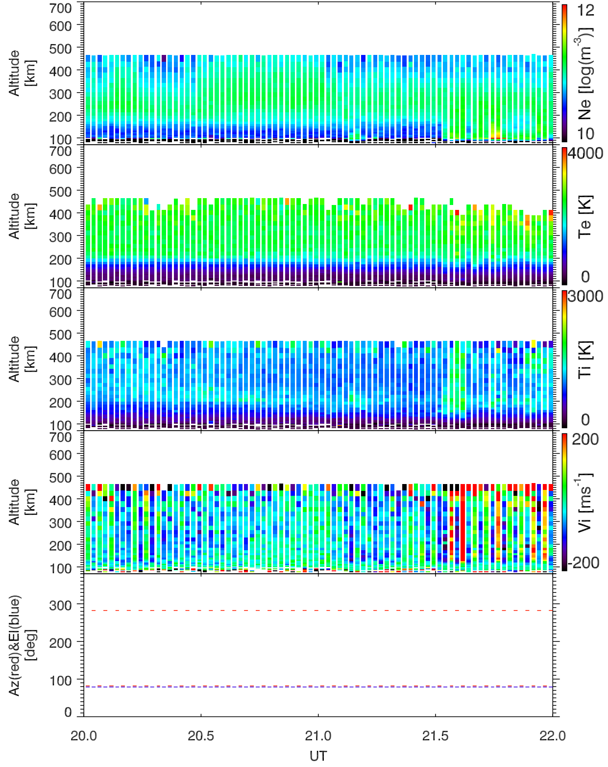
EISCAT 2007-05-24_20_22UT_ipy_ant@32m.
