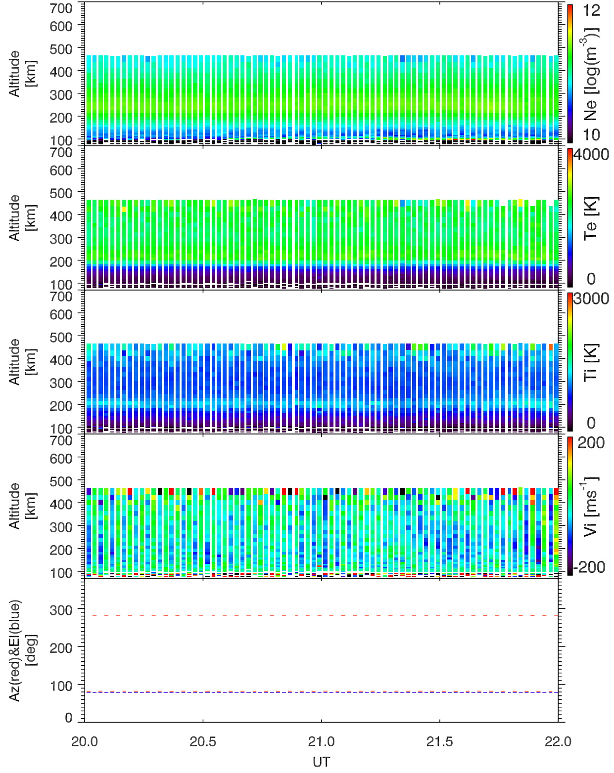
EISCAT 2007-06-07_20_22UT_ipy_ant@32m.
