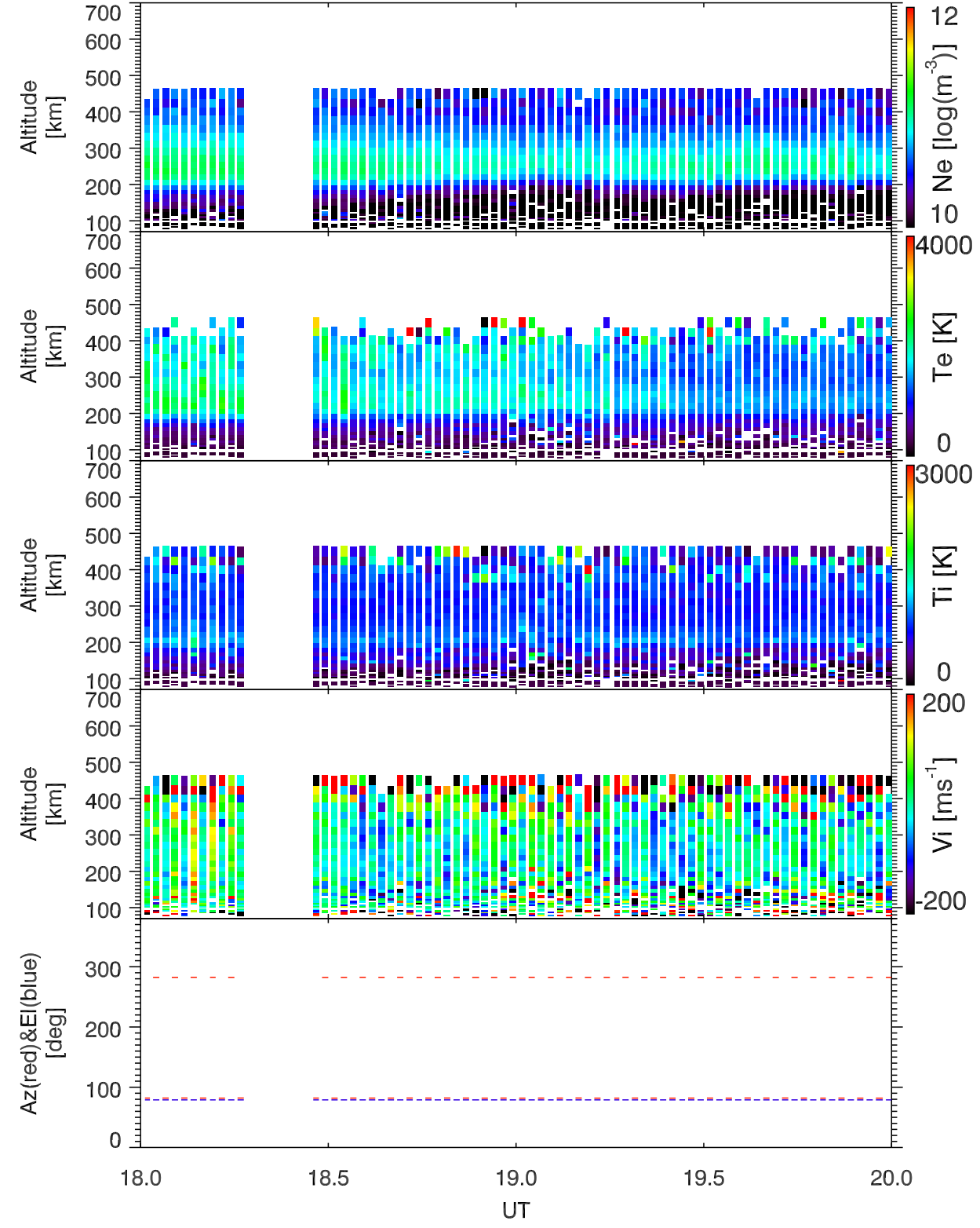
EISCAT 2007-09-13_18_20UT_ipy_ant@32m.
