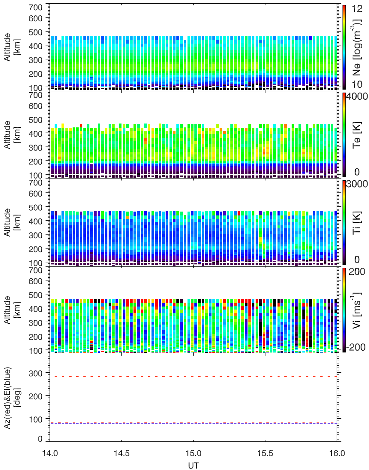
EISCAT 2007-09-27_14_16UT_ipy_ant@32m.
