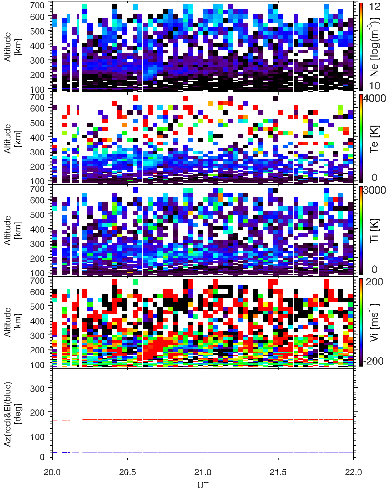
EISCAT 2008-01-26_20_22UT_tau0_120@32m.
