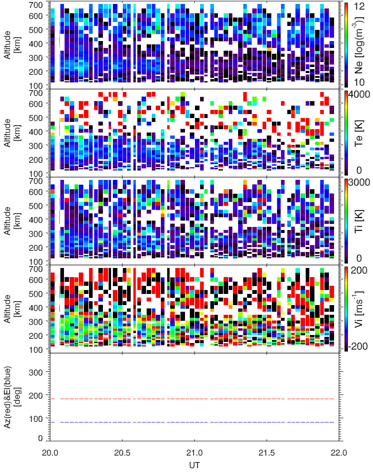
EISCAT 2008-01-26_20_22UT_tau0_120@42m.
