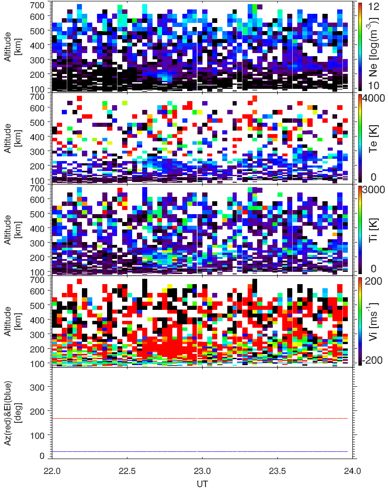
EISCAT 2008-01-26_22_24UT_tau0_120@32m.
