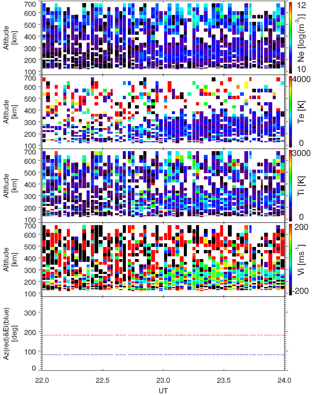
EISCAT 2008-01-26_22_24UT_tau0_120@42m.
