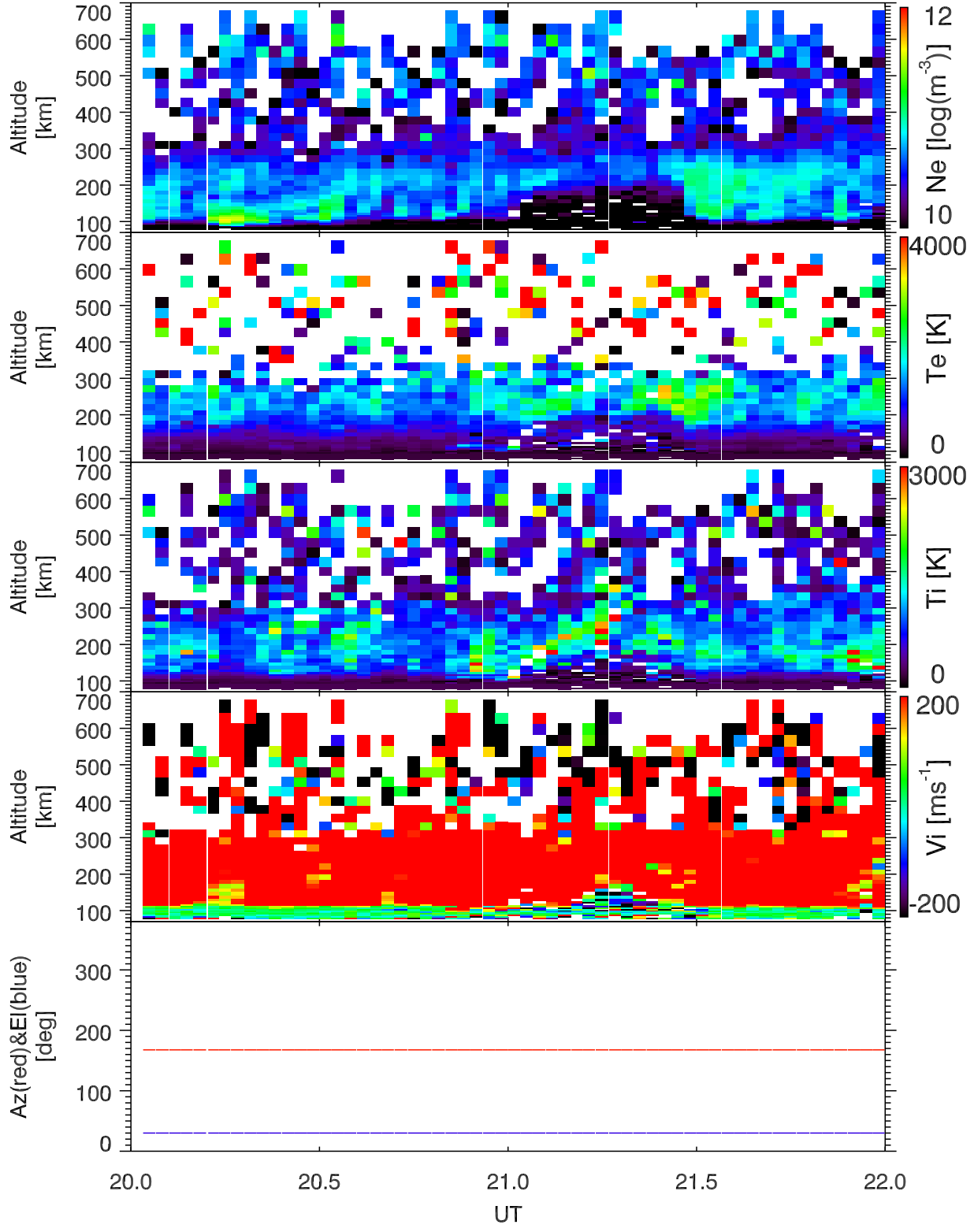
EISCAT 2008-01-27_20_22UT_tau0_120@32m.
