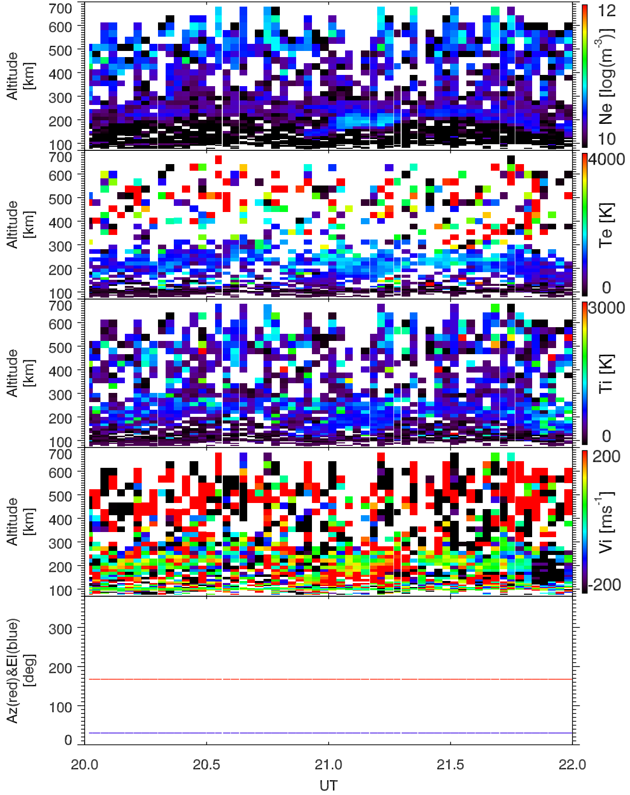
EISCAT 2008-01-30_20_22UT_tau0_120@32m.
