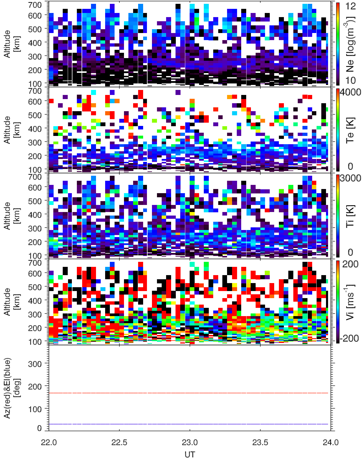
EISCAT 2008-01-30_22_24UT_tau0_120@32m.
