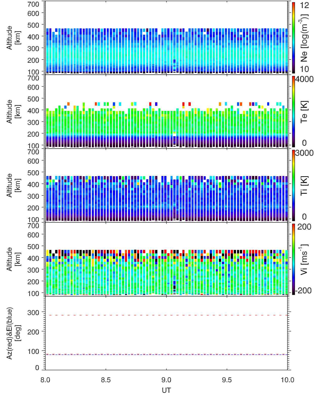
EISCAT 2008-05-09_08_10UT_ipy_ant@32m.
