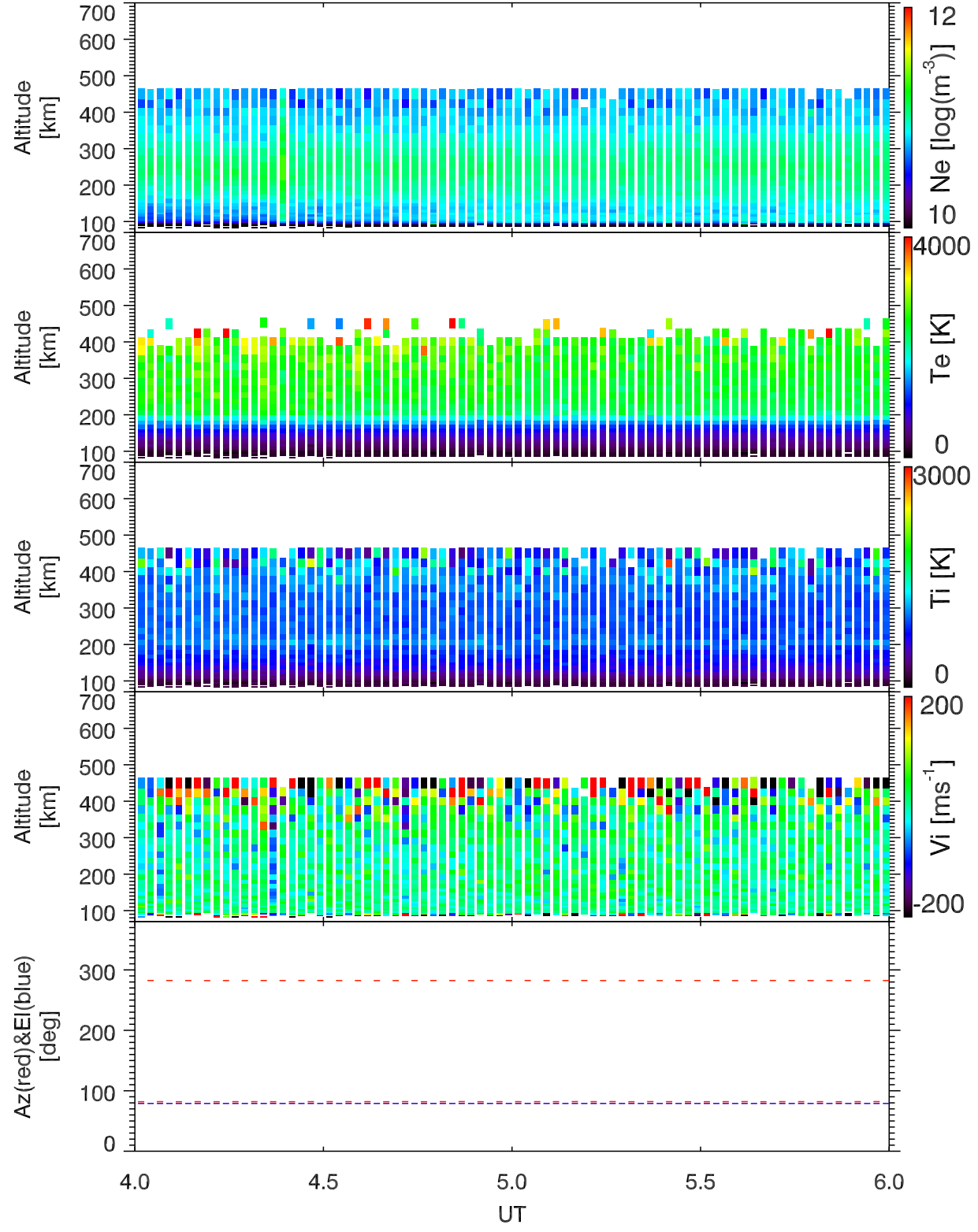
EISCAT 2008-05-23_04_06UT_ipy_ant@32m.
