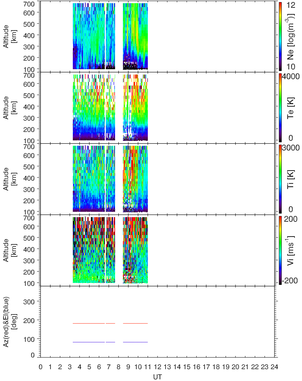
EISCAT 2000-02-07_00_24UT_gup3c_120@42m.
