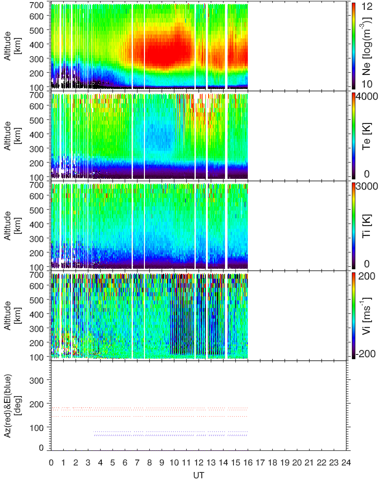
EISCAT 2000-03-20_00_24UT_gup3c_ant@32m.
