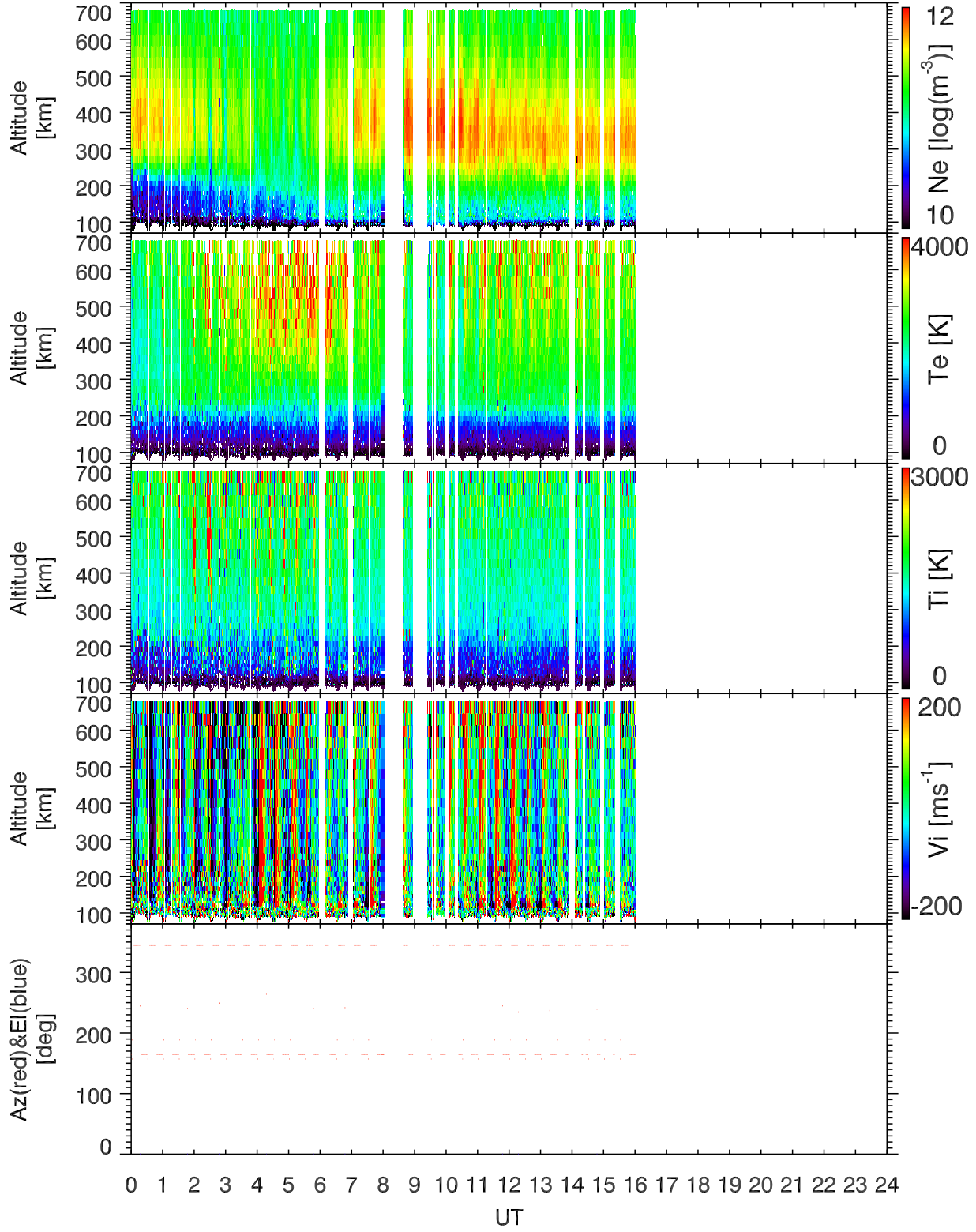
EISCAT 2000-04-13_00_24UT_tau0_ant@32m.
