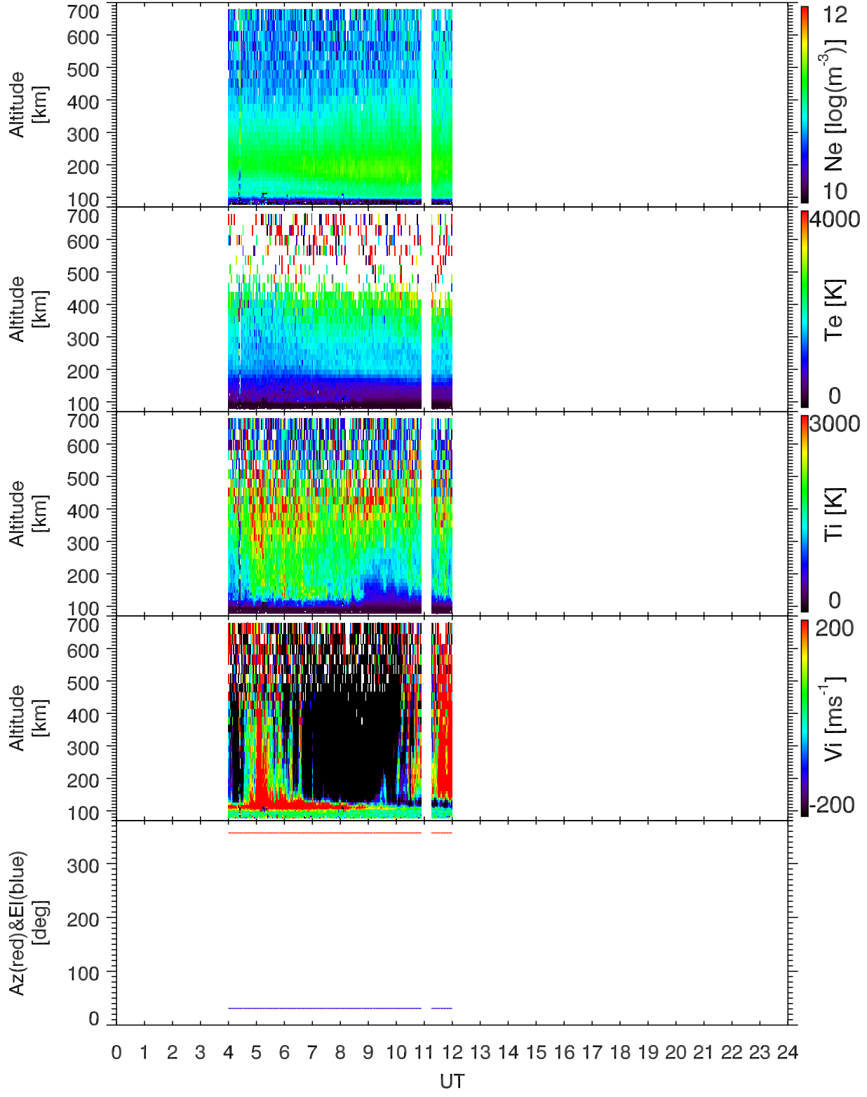
EISCAT 2000-07-16_00_24UT_tau0_120@32m.
