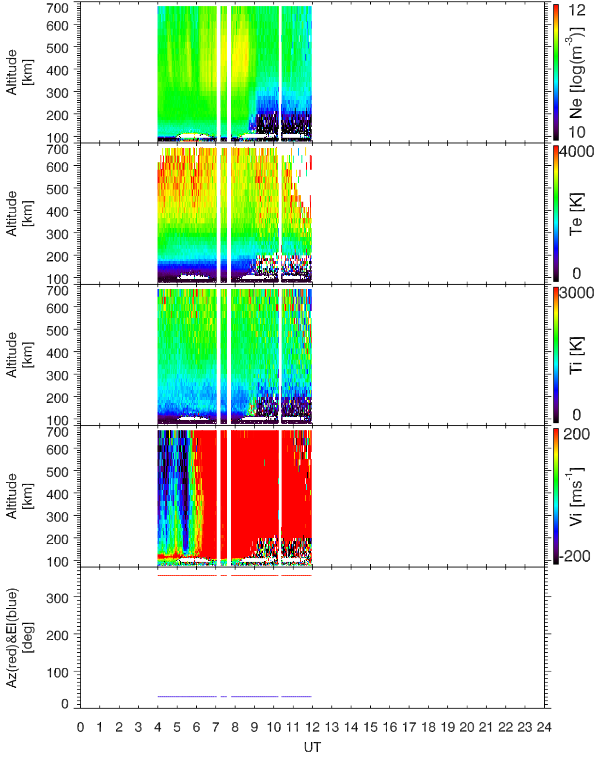
EISCAT 2000-07-20_00_24UT_tau0_120@32m.
