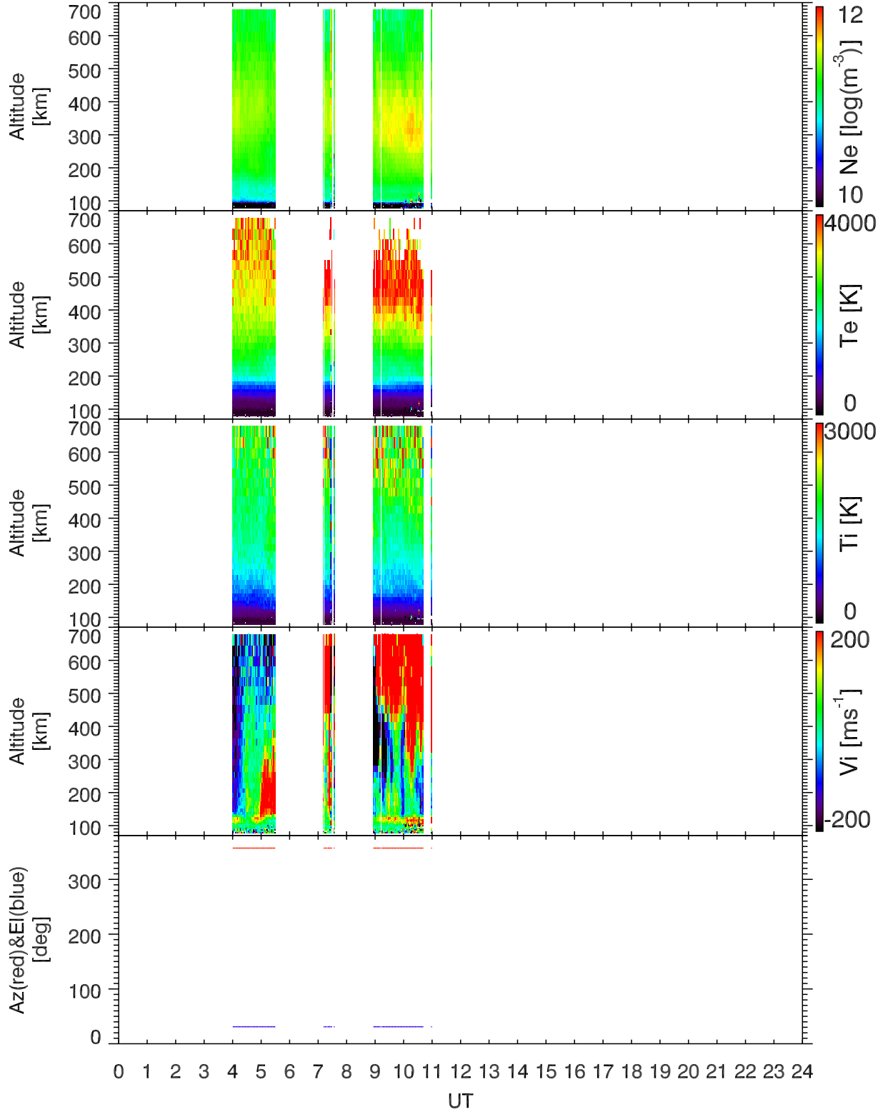
EISCAT 2000-07-23_00_24UT_tau0_120@32m.
