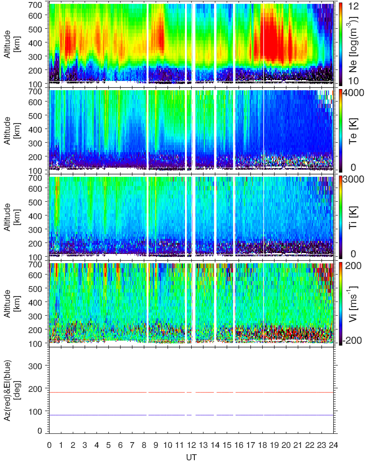
EISCAT 2001-11-14_00_24UT_tau0_120@42m.
