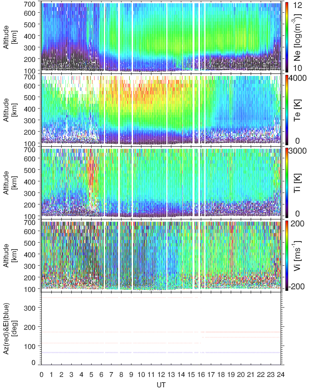
EISCAT 2002-10-10_00_24UT_tau0_ant@32m.
