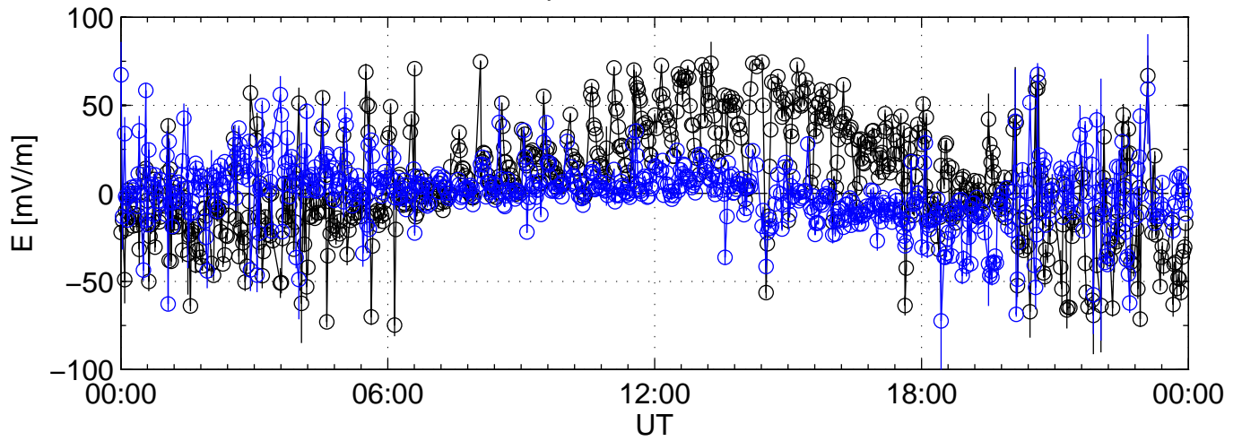
1991-09-26 kst cp3f 0000sec black:North, blue:East
