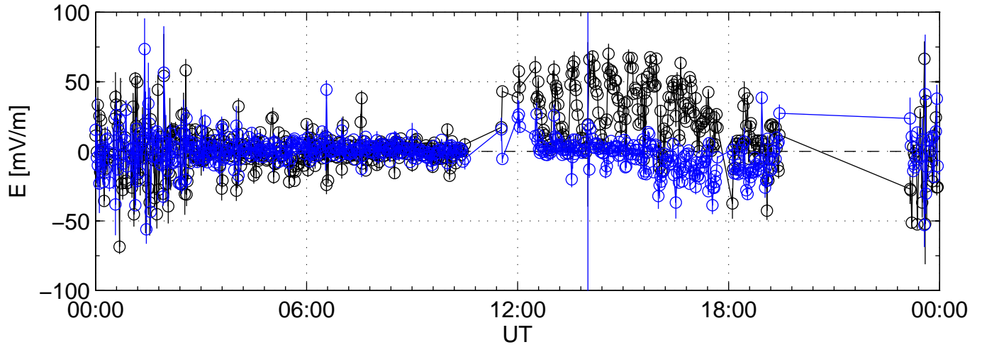
1999-04-21 kst cp3f 0000sec black:North, blue:East
