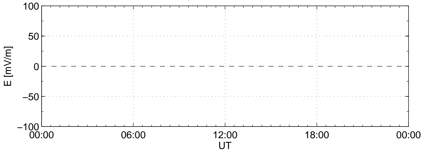
2001-02-16 kst cp1l 0060sec black:North, blue:East
