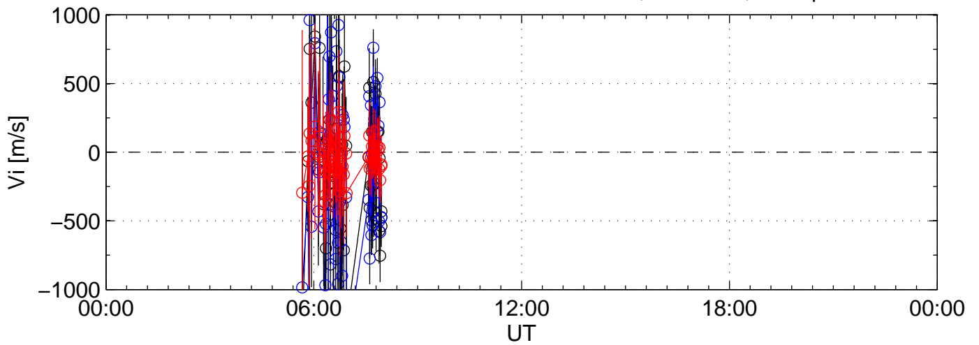
2002-01-25 kst tau2 0060sec black:North, blue:East
