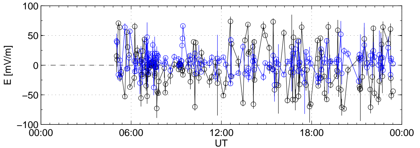
2004-05-18 kst tau1 0000sec black:North, blue:East
