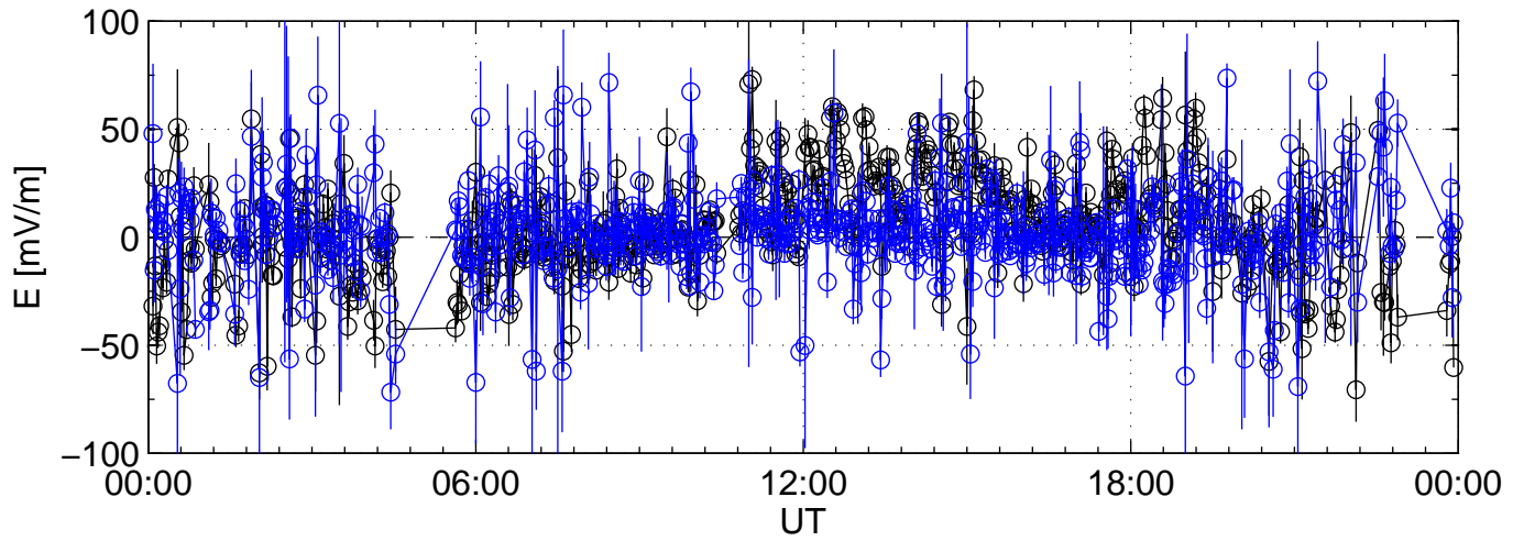
2005-04-20 kst tau1 0000sec black:North, blue:East
