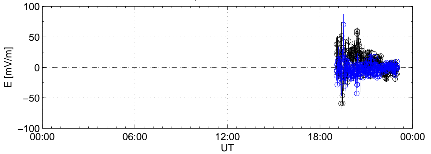
2006-10-08 kst t2pl 0060sec black:North, blue:East
