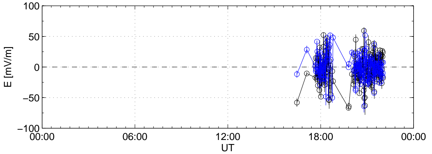
2006-10-17 kst t2pl 0060sec black:North, blue:East
