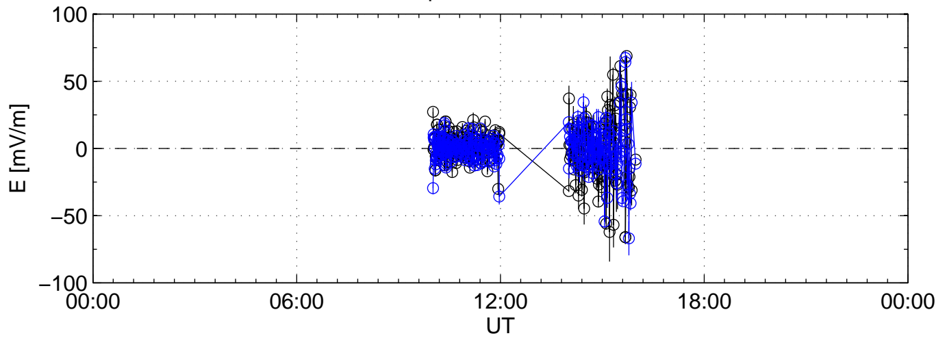
2006-12-16 kst t2pl 0060sec black:North, blue:East
