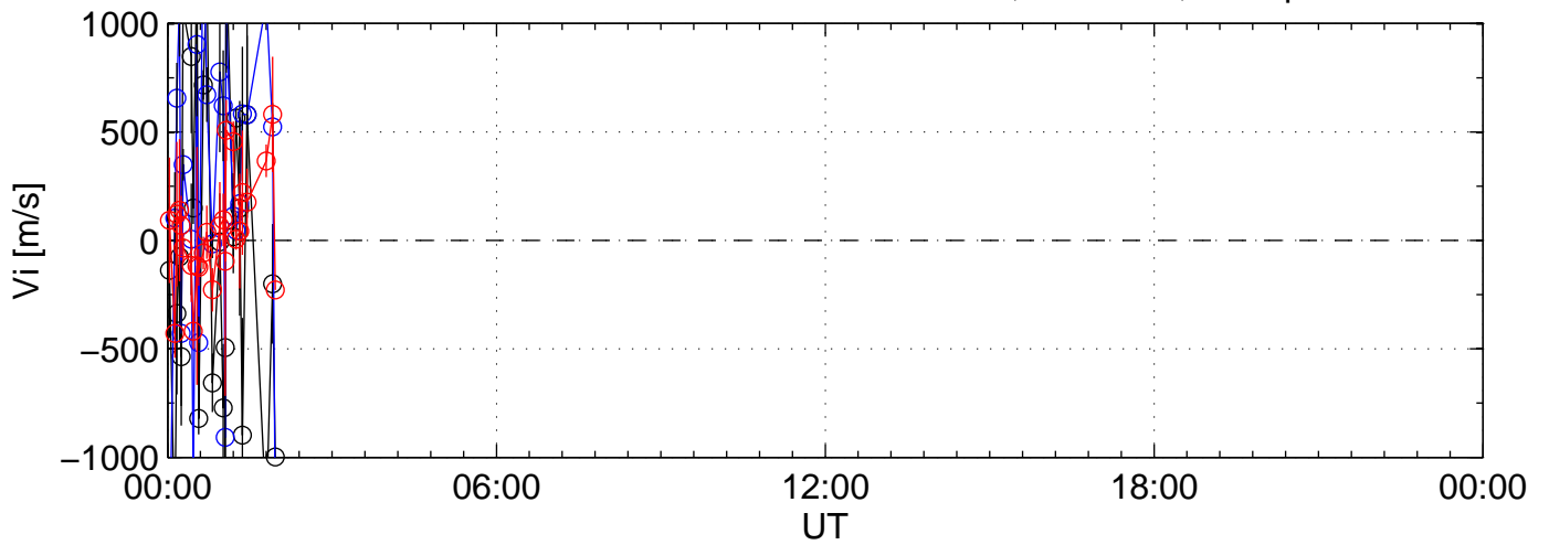
2007-11-22 kst arc1 0060sec black:North, blue:East
