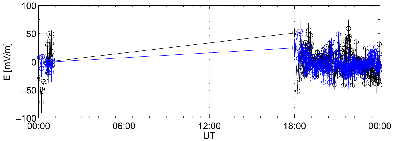
2008-02-02 kst t2pl 0060sec black:North, blue:East
