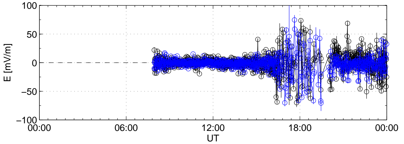
2010-01-26 kst beat 0000sec black:North, blue:East
