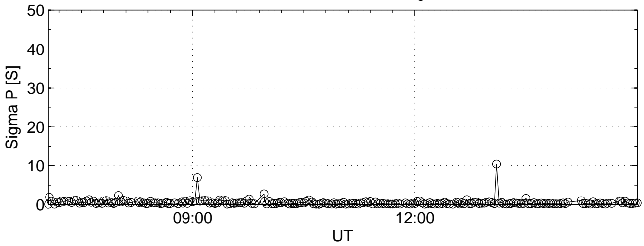
2001-01-07 tau0@42m Sigma P
