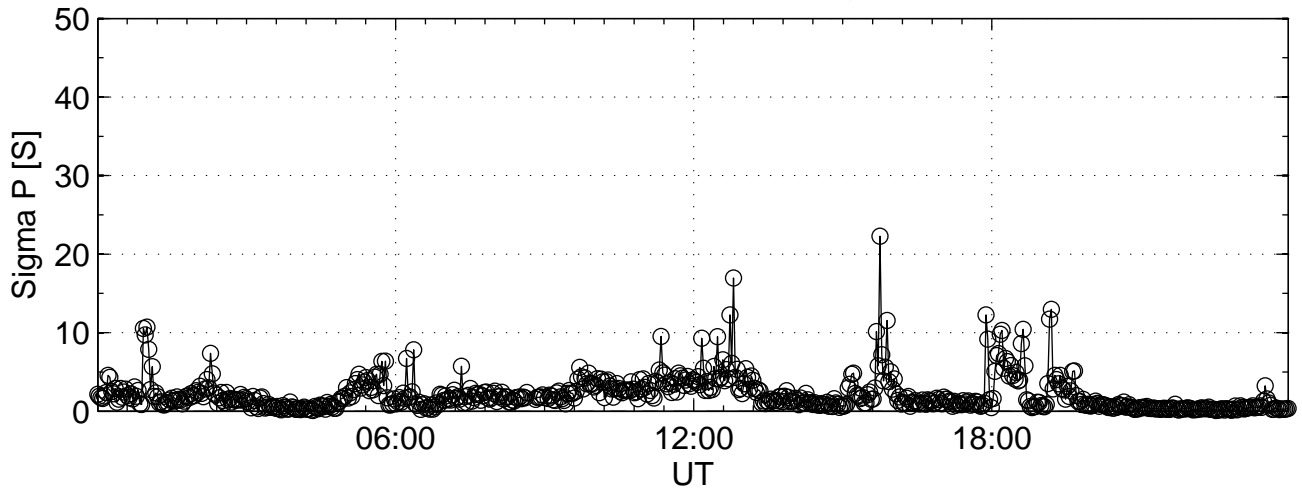
2002-10-26 tau0@42m Sigma P
