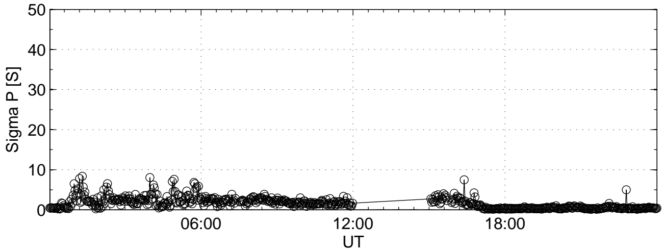
2002-11-14 tau0@42m Sigma P
