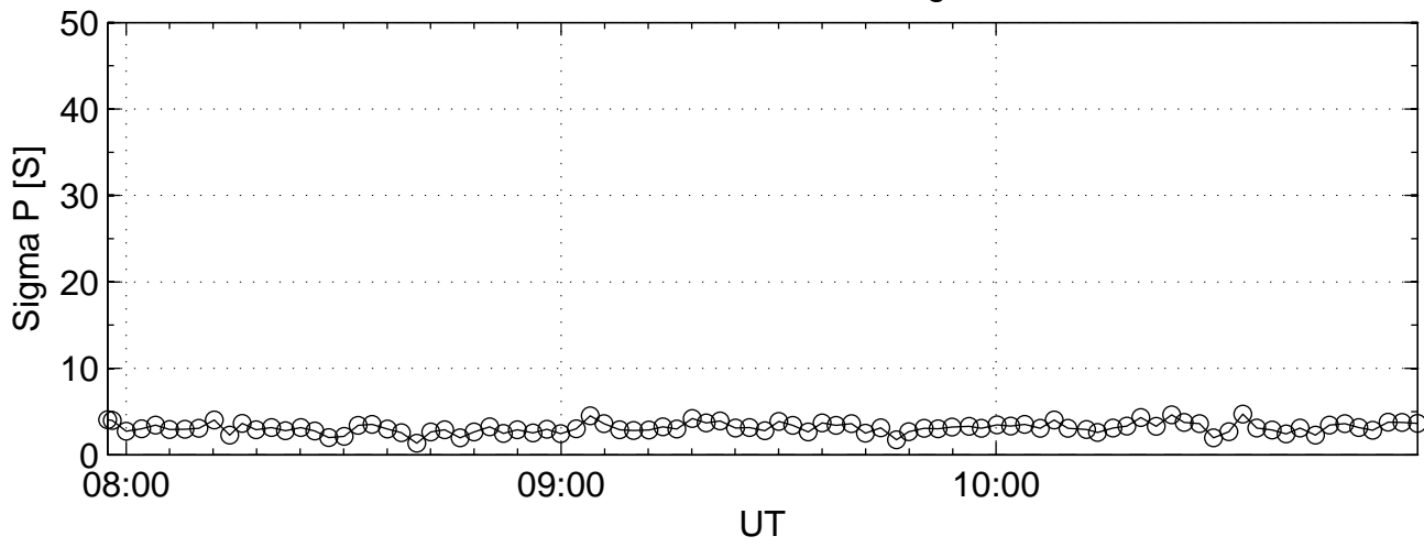
2004-05-05 tau0@42m Sigma P
