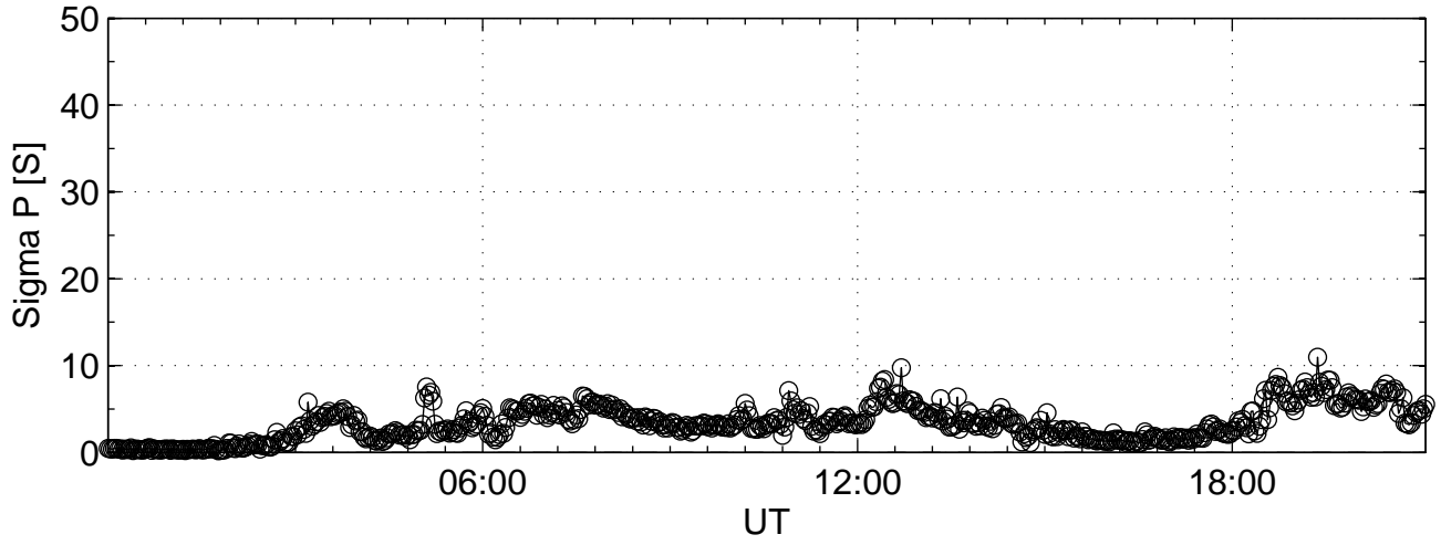
2004-11-07 steffe@42m Sigma P
