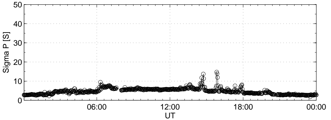
2007-06-19 ipy@42m Sigma P
