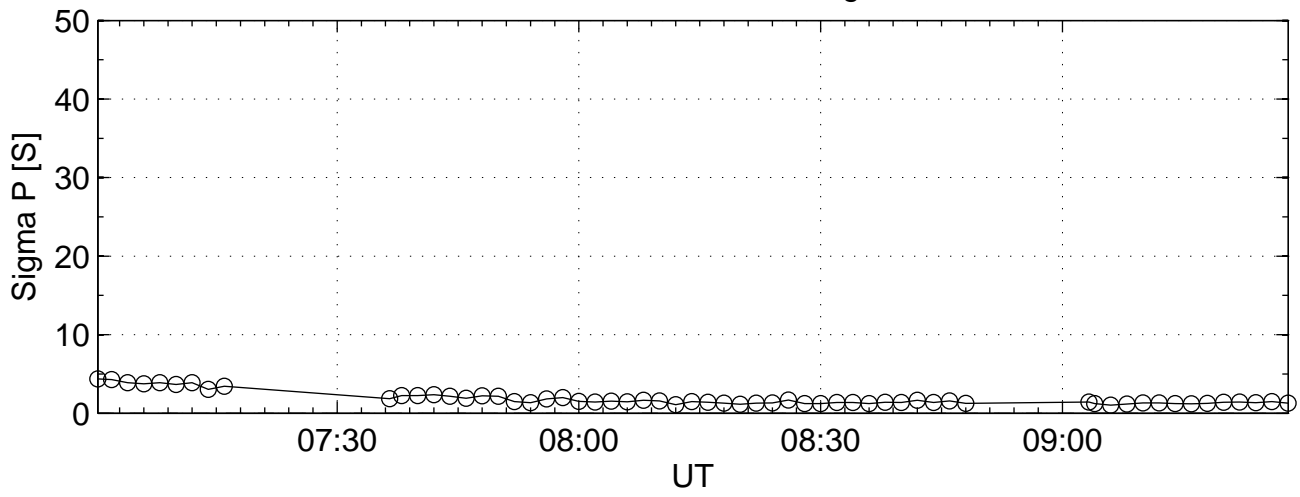
2008-11-10 tau7@42m Sigma P
