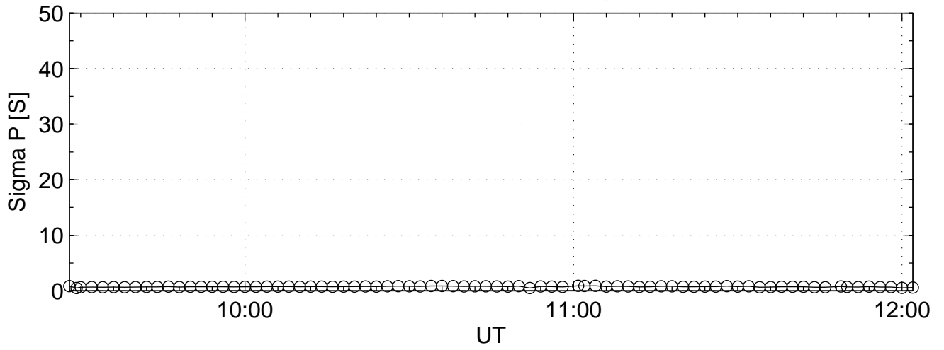
2007-12-09 tau2pl@uhf Sigma P
