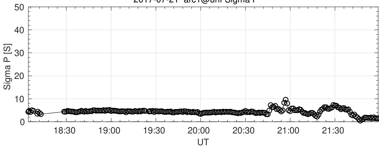
2017-07-21 arc1@uhf Sigma P
