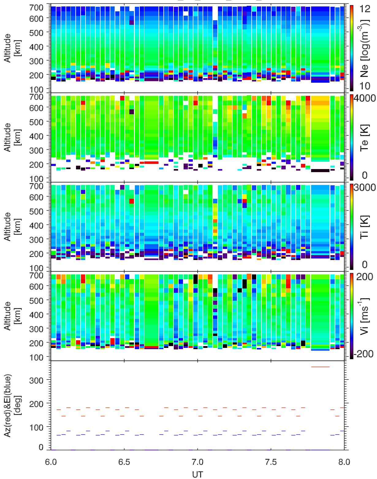
EISCAT 1998-03-24_06_08UT_gup0_ant@32m.
