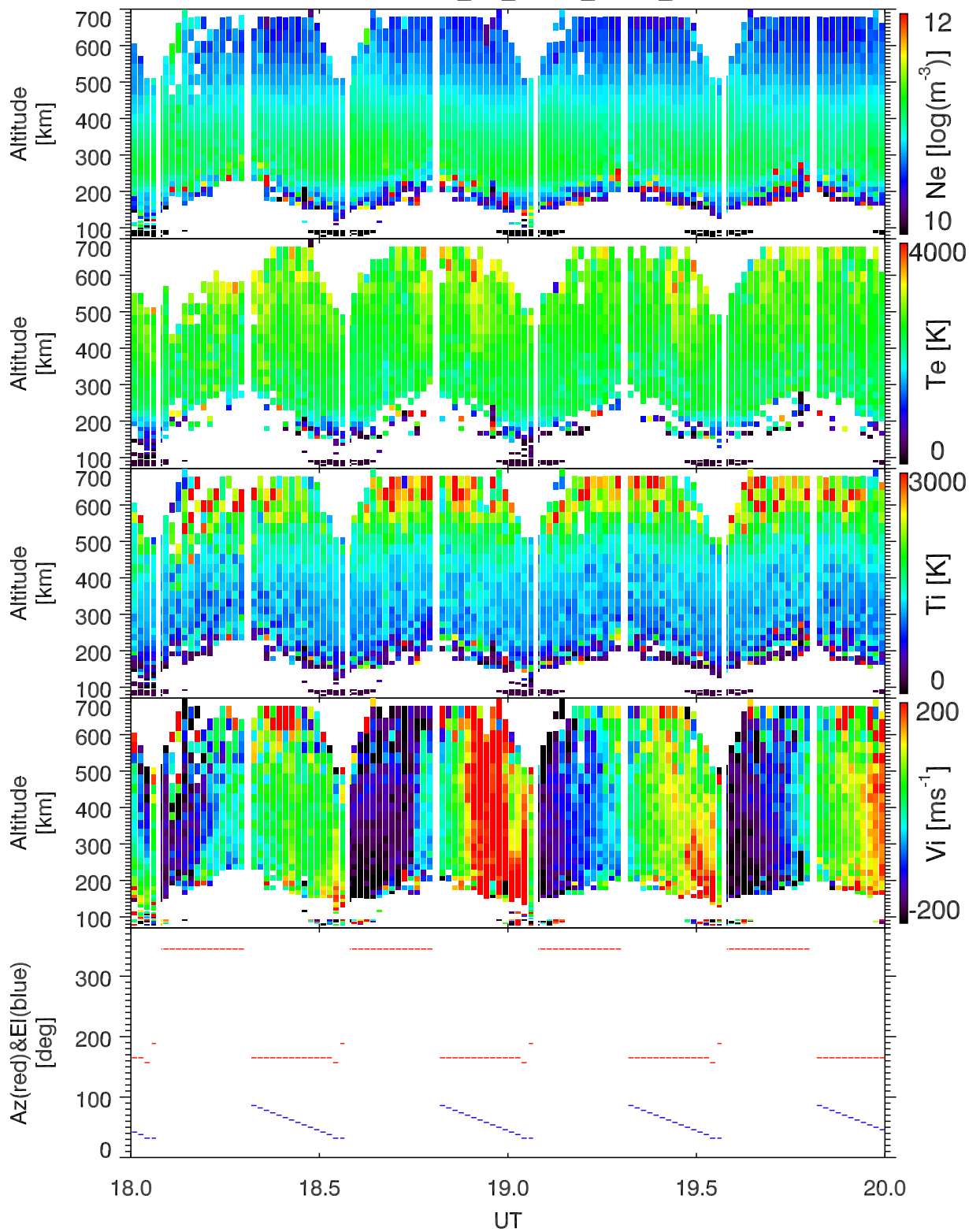
EISCAT 1998-04-28_18_20UT_gup0_ant@32m.
