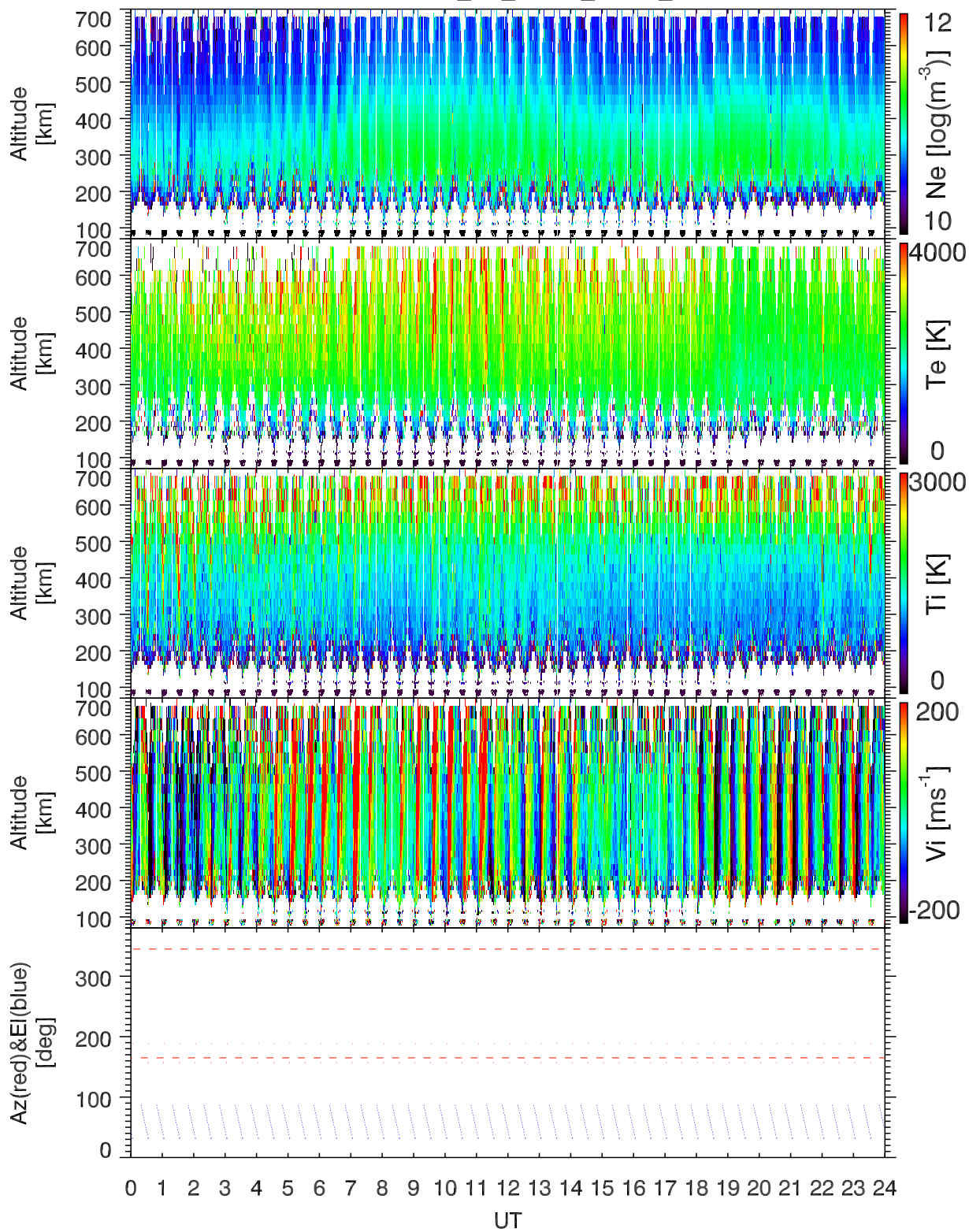
EISCAT 1998-04-29_00_24UT_gup0_ant@32m.
